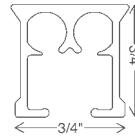
CCS® CONTRACT CORD SYSTEM Aluminum extrusion, white, powder coated, lubricated. Available in 25 white, 65 brown and 90 silver. All corded systems include child safety tension device.
