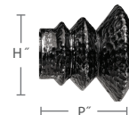
2120EVE-XX 3/4" Everest Finial H: 2" P: 1 7/8" $46.37 ea.
