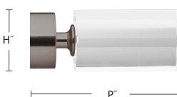
3035CIL-XX 1 3/8" Cylinder Finial H: 1 3/4" P: 4 1/4" $208.21 ea.
