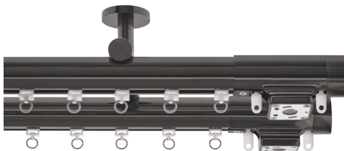
double traverse system, ceiling mount • ceiling bracket: 2 5/8" drop, 4 1/2" apart
